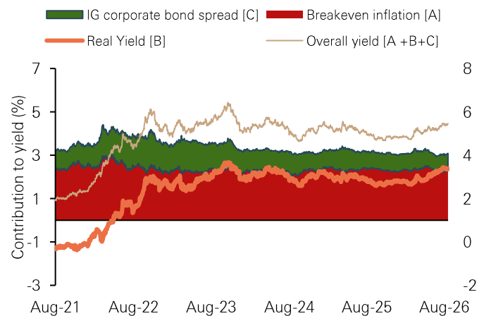
Chart 1: Yields are driven higher by real yields, while inflation expectations and spreads are stable
