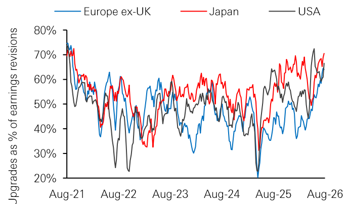
Chart 3: Earnings growth continues to broaden across markets, including Japan
